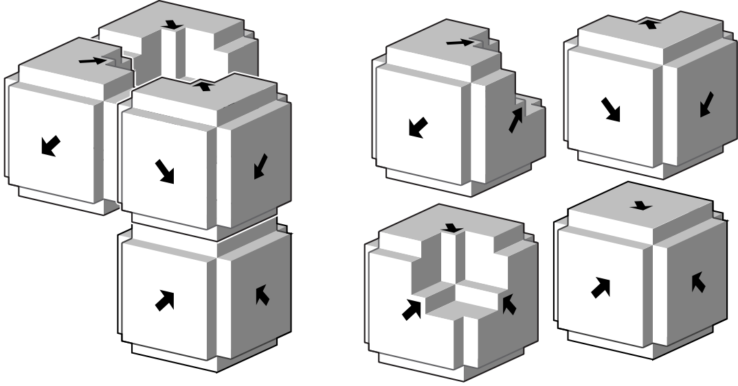
Figure 6: Several views of L
