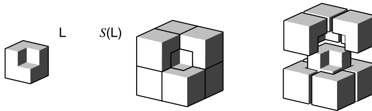
Figure 2: Constructing L_3
