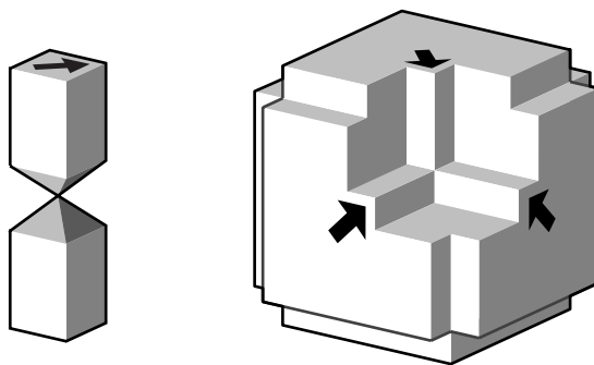
Figure 1: A pair of aperiodic tiles in \mathbb{E}^3
