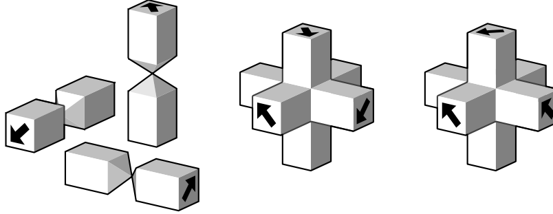
Figure 5: Several views of I, two typical X-tiles
