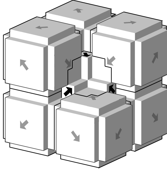
Figure 7: f(S^1(\mathbf{L}))
