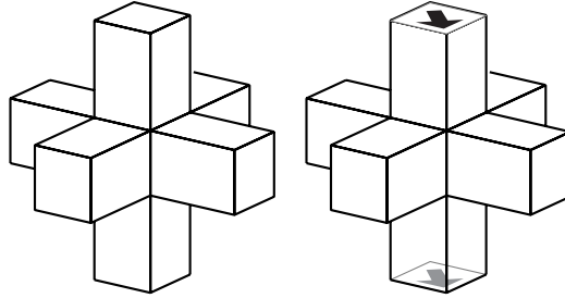
Figure 8: Two marked X tiles
