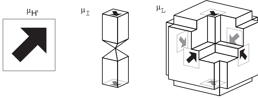
Figure 4: Constructing the markings on I and L
