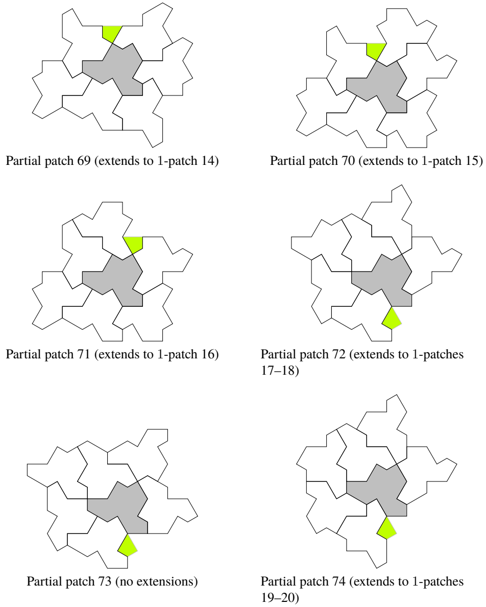
Figure B.2: Partial patches (part 10)
