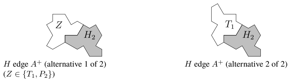
Figure 4.4: Between-cluster matching checks (part 1)
